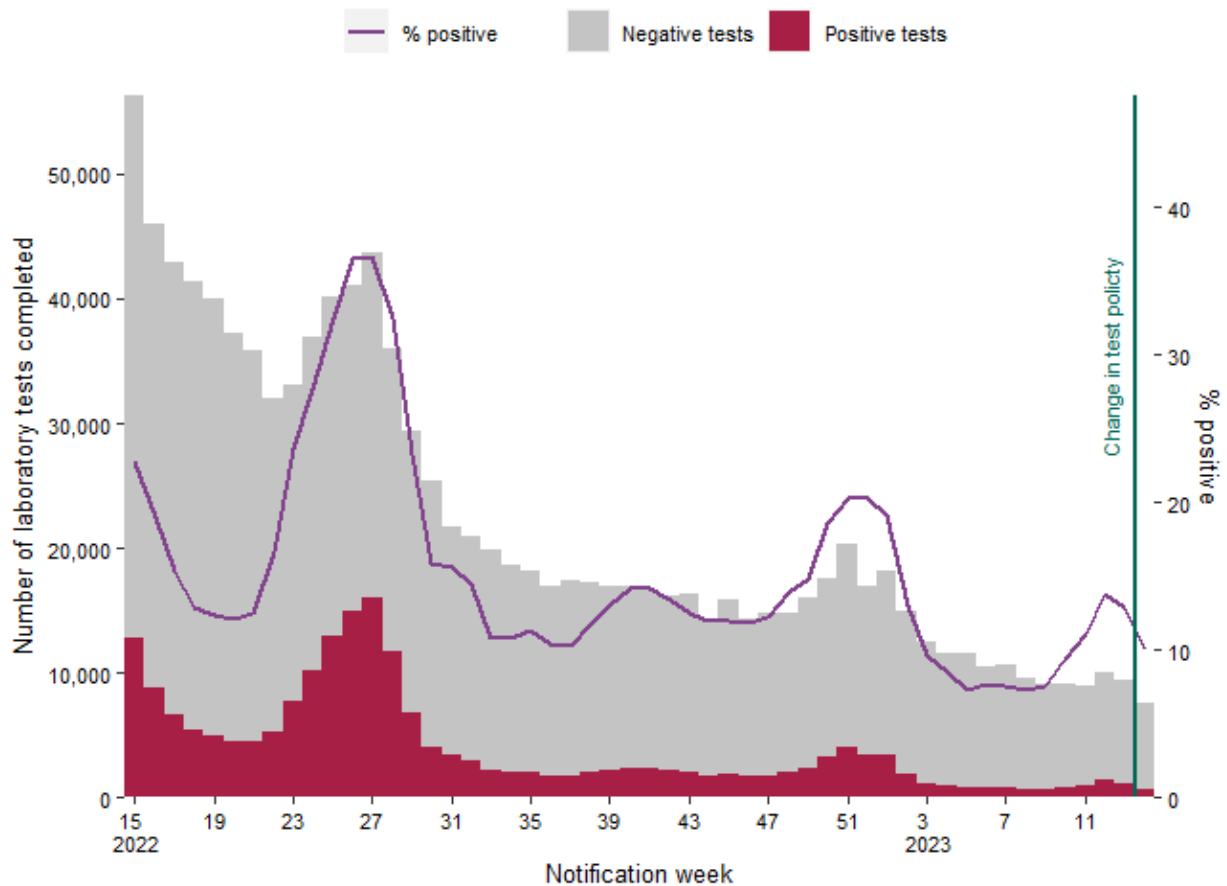
Figure 12: Number of completed laboratory tests by result and % positive tests 7 in Ireland between week 15, 2022 and week 14, 2023. Data source: Deloitte Ireland LLP 8, 9
