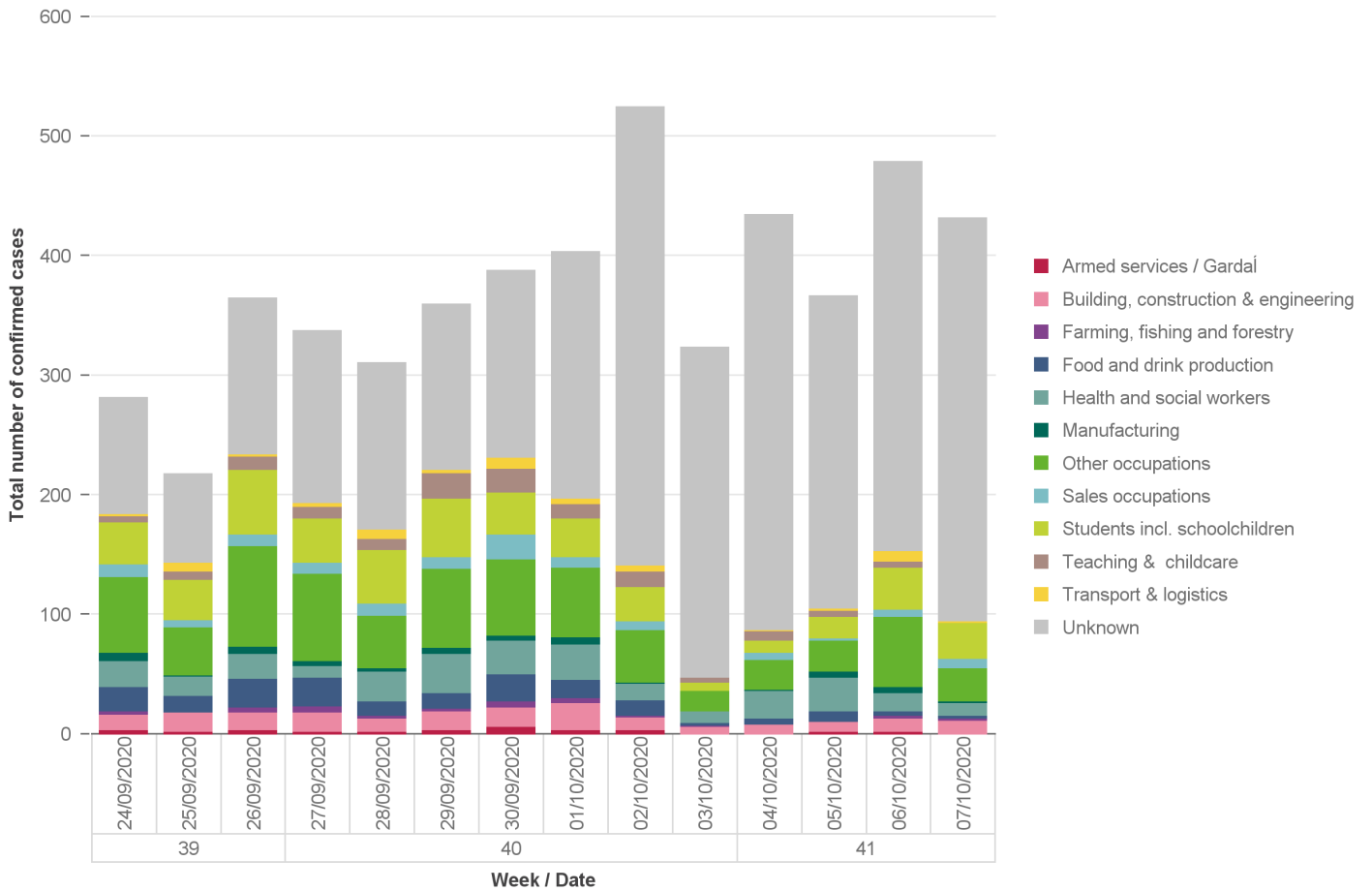
Figure 4: Number of confirmed COVID-19 cases notified in Ireland by date/week of notification and occupation* from 24/09/2020 to midnight 07/10/2020
